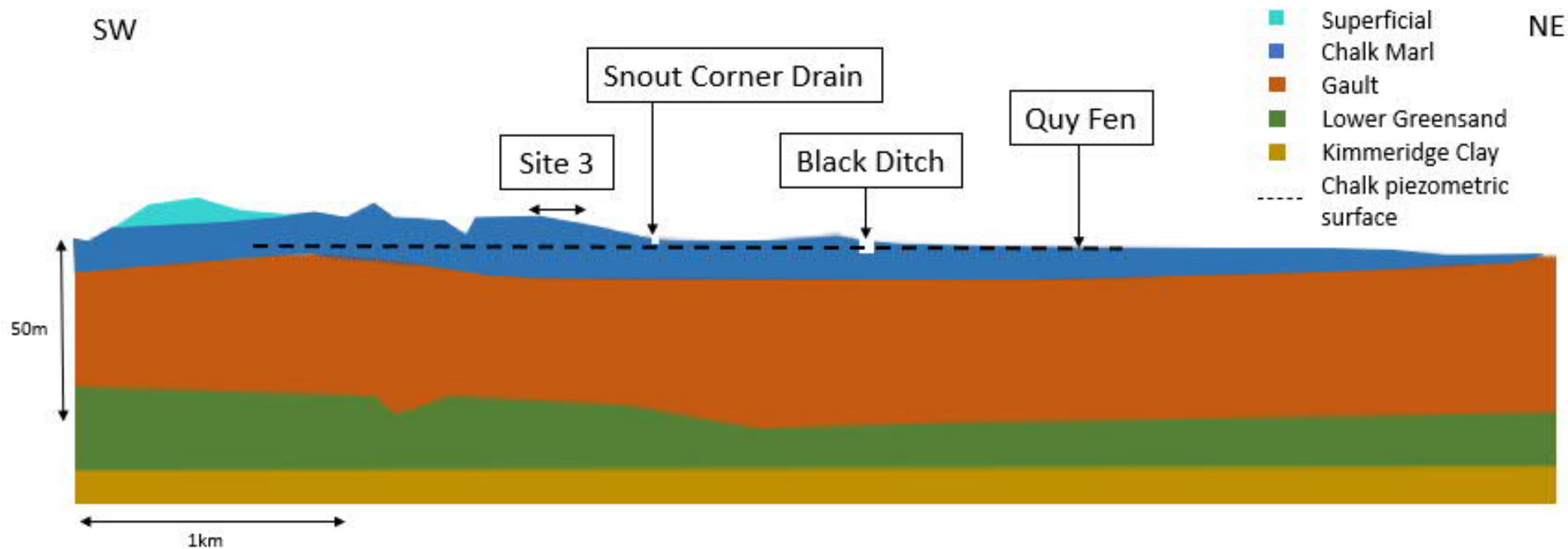
Figure A.12: SW/NE cross section beneath Site 3
