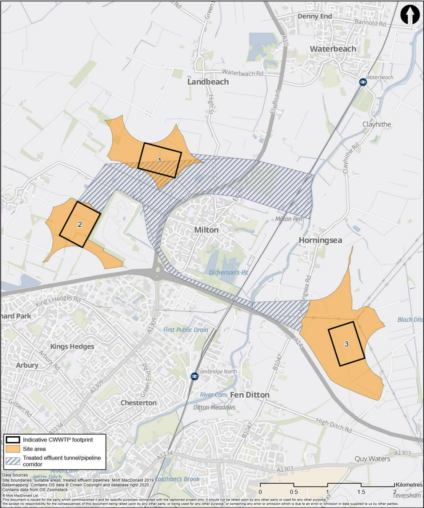
Figure A.16: Treated effluent transfer tunnel/pipeline corridors
